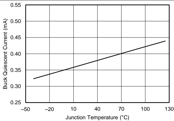
Figure 1. TPS562201 Supply Current vs Junction Temperature
