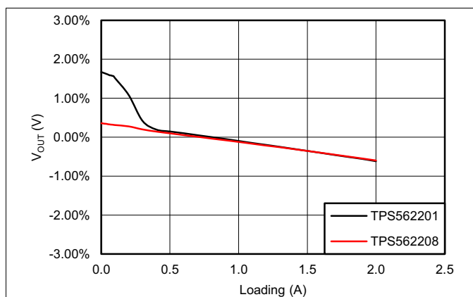
Figure 20. Load Regulation, V_{\text{IN}} = 5 \text{ V}
