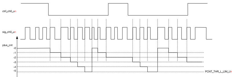
Figure 18: PULSE_CNT Downcounting Diagram
