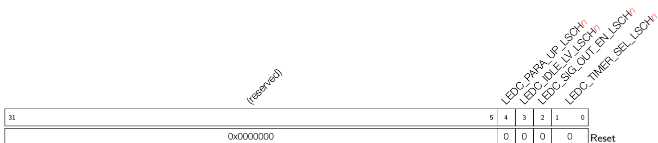
Register 5.6: LEDC_LSCH n _CONF0_REG ( n : 0-7) (0xBC+0x10* n )
