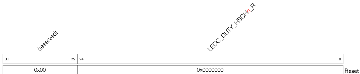
Register 5.5: LEDC_HSCH n _DUTY_R_REG ( n : 0-7) (0x2C+0x10* n )
