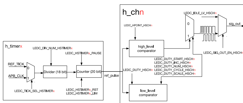
Figure 11: LED_PWM High-speed Channel Diagram
