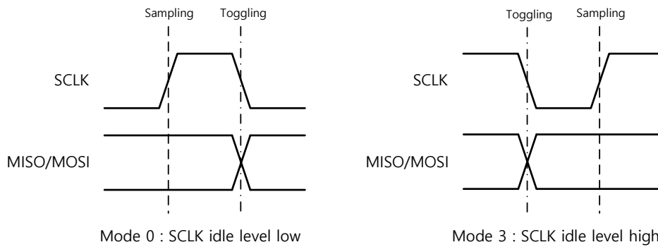
Figure 6. SPI Mode 0 & 3
