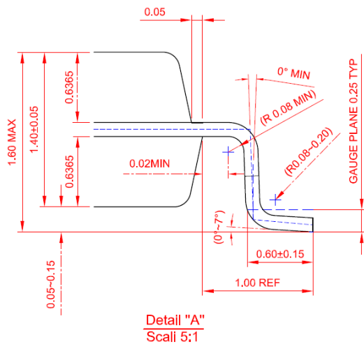
Figure 27. Package Dimensions
