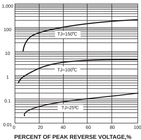
FIG. 4-TYPICAL REVERSE CHARACTERISTICS
